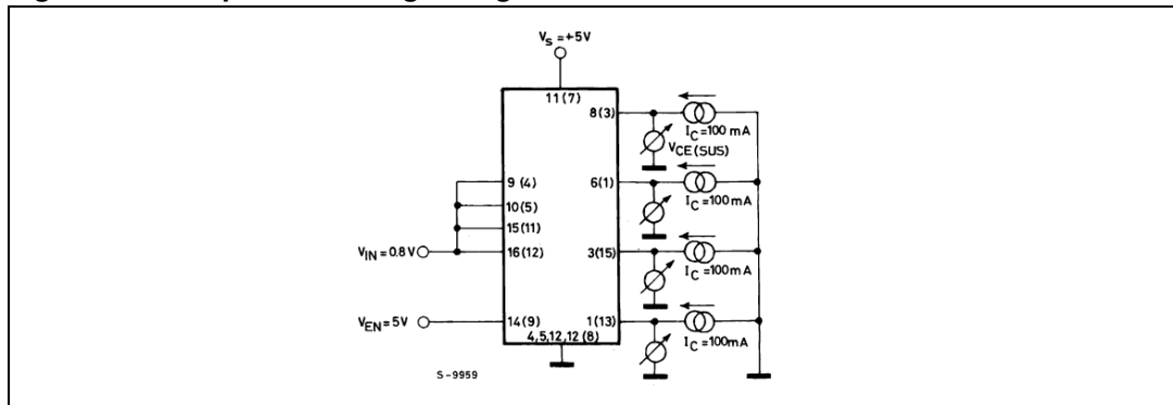
Figure 4. Output sustaining voltage
